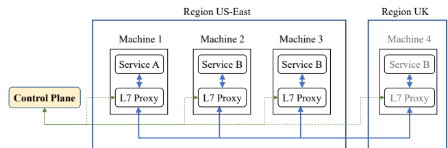
Figure 1: Sidecar-proxy-based service mesh.
